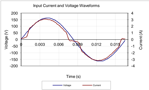
Input AC Current Waveform (ITHD = 11.07%, 50% Load)
