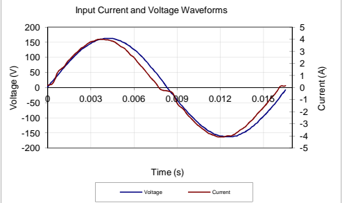
Input AC Current Waveform (ITHD = 7.92%, 50% Load)
