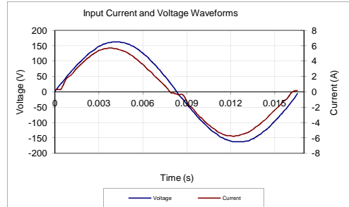
Input AC Current Waveform (ITHD = 8.85%, 50% Load)
