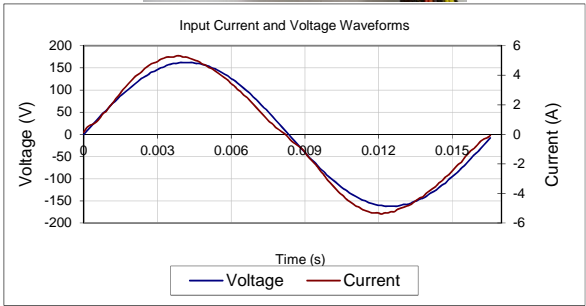
Input AC Current Waveform (ITHD = 0.45%, 50% Load)
